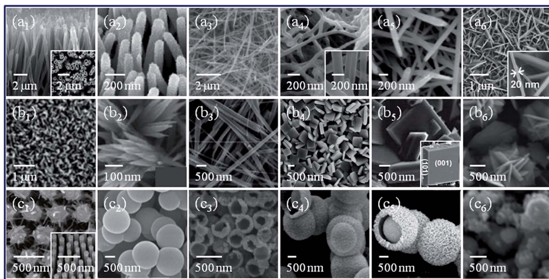
Fig. 11 SEM micrographs of anatase-TiO 2 nanostructures: (a 1 and a 2 ) nanotubes, (a 3 and a 4 ) nanofibres, (a 5 ) nanorods, (a 6 ) nanorods with nanoflakes, (b 1 ) nanoribbon arrays, (b 2 ) nanoribbons, (b 3 ) nanowires, (b 4 –b 6 ) nanosheets, (c 1 ) 3D network, (c 2 ) nanospheres, (c 3 ) nanospheres, (c 4 and c 5 ) nanospheres and (c 6 ) nanoparticles. Insets (a 1 , a 4 , a 6 , b 5 and c 1 ) provide the corresponding higher magnification images. Ref: [a 1 , a 2 ], 50 [a 3 ], 329 [a 4 ], 50 [a 5 ], 269 [a 6 ], 270 [b 1 ], 330 [b 2 ], 271 [b 3 ], 50 [b 4 ], 292 [b 5 ], 41 [b 6 ], 331 [c 1 ], 50 [c 2 ], 274 [c 3 ], 274 [c 4 , c 4 and c 5 ], 273 [c 6 ]. 275 (a 1 , a 2 , a 4 , b 3 and c 1 ) are reprinted with permission from ref. 50. Copyright 2014. American Chemical Society. (a 3 ) is reprinted with permission from ref. 329. Copyright 2005. Elsevier. (a 5 ) is reprinted with permission from ref. 269. Copyright 2013. The Royal Society of Chemistry. (a 6 ) is reprinted with permission from ref. 270. Copyright 2012. The Royal Society of Chemistry. (b 1 ) is reprinted with permission from ref. 330. Copyright 2004. The Royal Society of Chemistry. (b 2 ) is reprinted with permission from ref. 271. Copyright 2011. American Chemical Society. (b 4 ) is reprinted with permission from ref. 292. Copyright 2009. American Chemical Society. (b 5 ) is reprinted with permission from ref. 41. Copyright 2009. American Chemical Society. (b 6 ) is reprinted with permission from ref. 331. Copyright 2011. John Wiley and Sons. (c 2 , c 4 and c 5 ) are reprinted with permission from ref. 273. Copyright 2007. American Chemical Society. (c 3 ) is reprinted with permission from ref. 274. Copyright 2013. The Royal Society of Chemistry. (c 6 ) is reprinted with permission from ref. 275. VBRI Press.
