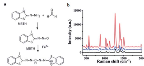
Fig. 16 (a) Derivatization reaction between FA and MBTH hydrochloride. (b) Raman spectra of MBTH with Au/SiO 2 NPs (1), the derivative product before (2) and after (3) the addition of Au/SiO 2 NPs at 785 nm excitation wavelength (this figure has been adapted from ref. 71 with permission from RSC).
