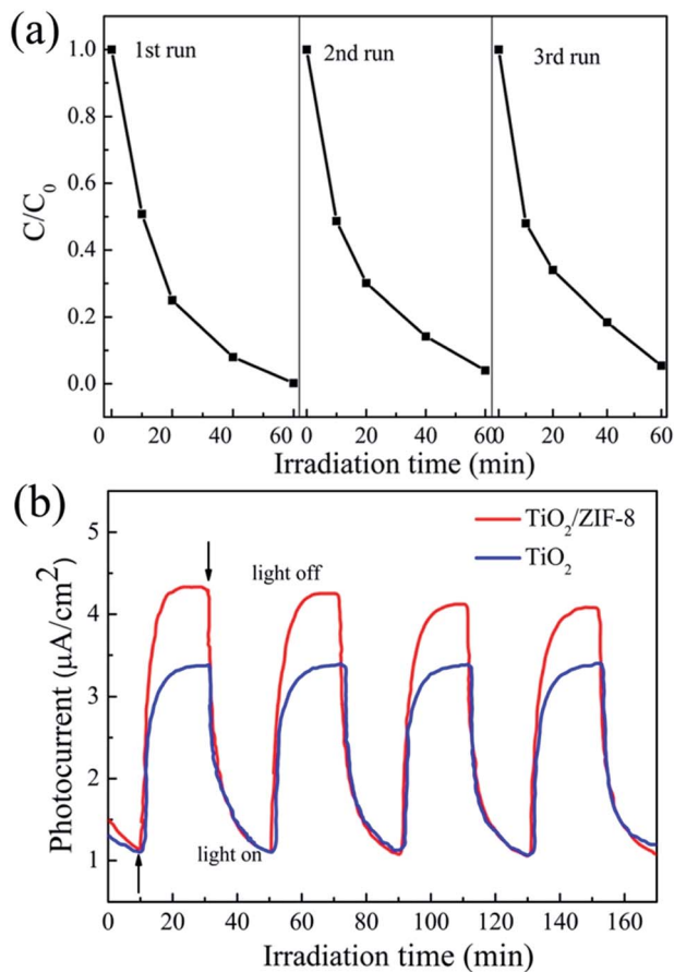
Fig. 7 (a) Recycling test on \text{TiO}_2/\text{ZIF-8} for photocatalytic reduction of \text{Cr}(\text{vi}) . (b) Transient photocurrent response of \text{TiO}_2/\text{ZIF-8} and \text{TiO}_2 in 0.1 M \text{Na}_2\text{SO}_4 aqueous solution.
