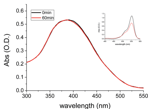
Fig. 6 Absorption changes of BBTA in PBS-mPEG 550 (95 : 5, v/v, 10 \mu\text{M} ) with 365 nm light irradiation (periods: 0 and 60 min; power: 36 W, energy: 3.7 \text{mW cm}^{-2} ). Inset: absorption change of rhodamine B in PBS-mPEG 550 (95 : 5, v/v, 10 \mu\text{M} ) with 365 nm light irradiation (periods: 0 and 60 min; power: 36 W, energy: 3.7 \text{mW cm}^{-2} ).
