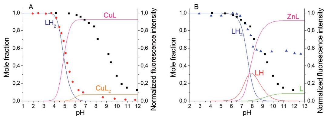
Fig. 3 Fluorescence emission pH titration curves of compound 5 (10 \mu\text{M} , \lambda_{\text{ex}} = 472 \text{ nm} , \lambda_{\text{em}} = 552 \text{ nm} ) in water in the absence (black \blacksquare ) or presence of 1 equivalent of metal ion, (A) Cu(II) (red \bullet ) and (B) Zn(II) (blue \blacktriangle ), and mole fraction distribution diagrams for the various species of this ligand under these conditions (solid lines).
