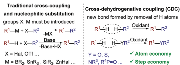
Scheme 1 Traditional and cross-dehydrogenative coupling.
