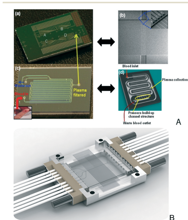
Fig. 2 A) Si nanowire biosensing platform (a and b) and integrated plasma filtration microfluidic (c and d) for cardiac biomarker quantification (reprinted from ref. 17, copyright 2011, with permission from Elsevier) and B) glass microfluidic interfacing (Dolomite Ltd.). 32
