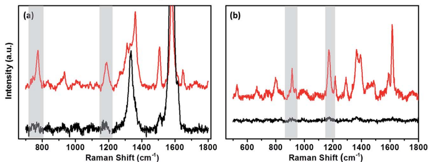
Fig. 3 Raman spectra of (a) 0.1 mM rhodamine-6G in ethanol on BPPG with SHINs (red) and without SHINs (black); (b) 0.1 mM malachite green in water on GC with SHINs (red) and without SHINs (black). Shaded areas indicate the peaks analysed for EF calculations.
