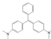
Malachite green
