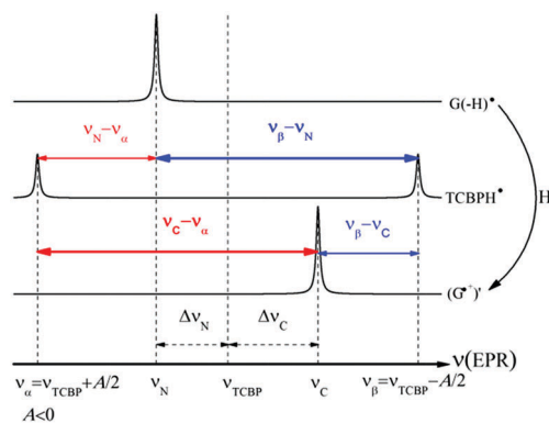
Scheme 1 Schematic representation of triplet-singlet interconversion based on the EPR spectra of \text{G}(\text{H})^{\bullet} (top), \text{TCBPH}^{\bullet} (middle), and (\text{G}^{\bullet+})' (bottom). Only a single spin-1/2 nucleus in \text{TCBPH}^{\bullet} with negative HFCC is considered.
