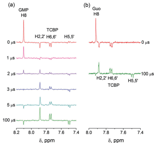
Fig. 1 (a) 1 H CIDNP spectra, detected in the photoreaction of 2 mM 3,3',4,4'-tetracarboxy benzophenone and 20 mM guanosine-5'-monophosphate in 50 mM sodium phosphate buffer at pH 6.9 at variable time delays after the laser pulse. The delays are ascending from 0 (top) to 100 μs (bottom spectrum). (b) 1 H CIDNP spectra detected in the photoreaction of 2 mM 3,3',4,4'-tetracarboxy benzophenone and 2 mM guanosine in 50 mM sodium phosphate buffer at pH 6.9. The upper spectrum was taken immediately after the laser pulse, and the lower spectrum at 100 μs after the laser pulse.
