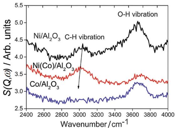
Fig. 18 INS spectra of methane reforming catalysts after dry reforming at 875 K for six hours. Reproduced from ref. 81 by permission of the PCCP Owner Societies.
