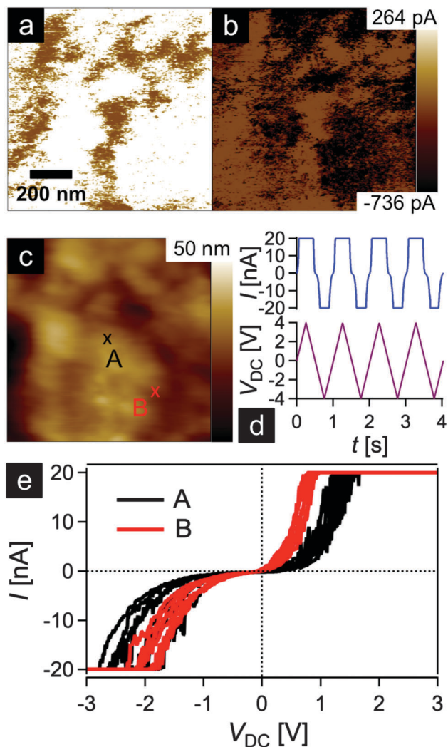
Fig. 10 Conductive AFM experiment performed on a melt-shear organized particle film thermally treated at 1500 °C. (a and b) Current maps applying +1V (a) and -1V (b) to the sample surface, respectively, and the corresponding topography image (c). (d) Current measured during four triangular voltage cycles at position A marked in (c). (e) Current-voltage spectroscopy curves conducted at two different sample positions marked by A (black curve) and B (red curve) in the topography image of (c). Each curve consists of four consecutive cycles as shown by the current versus time and voltage versus time graphs (d).
