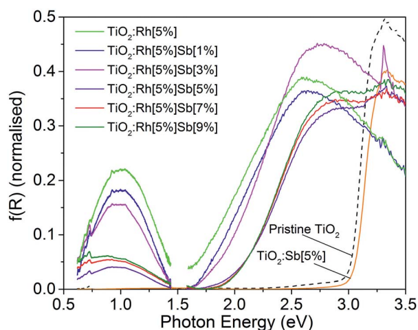
Fig. 6 Absorption spectra for all \text{TiO}_2:\text{Rh}[5\%]\text{Sb}[X\%] powders. A decrease in photon energy required for photoexcitation is exhibited by all Rh doped samples by comparison to pristine \text{TiO}_2 . An additional absorption around 1.0 eV, which can be attributed to a valence band to \text{Rh}^{4+} t_{2g} transition, is prominent in samples containing \text{Rh}^{4+} . The reduction in intensity of this feature is evidence of the suppression of \text{Rh}^{4+} in samples of higher \text{Sb}^{5+} concentration.
