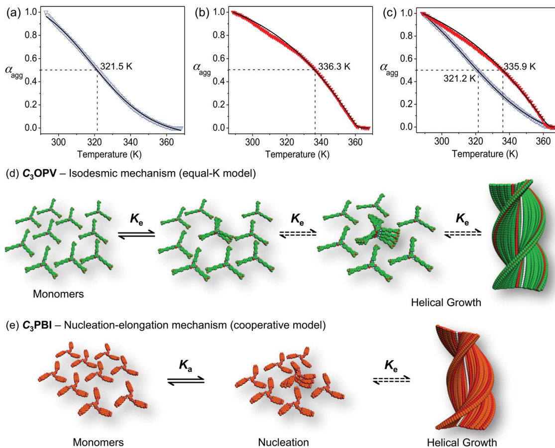
Fig. 2 Plot of the fraction of aggregates ( \alpha_{\text{agg}} ) against temperature for (a) C_3\text{OPV} and (b) C_3\text{PBI} individual assemblies, and (c) for C_3\text{OPV} and C_3\text{PBI} as a 1 : 1 mixture in toluene ( 1 \times 10^{-4} M). C_3\text{OPV} ( \Delta ), C_3\text{PBI} ( \nabla ) and curve fitting (—). Absorbance was monitored at 425 and 527 nm for C_3\text{OPV} and C_3\text{PBI} , respectively, with a rate of cooling of 1 \text{ K min}^{-1} . Schematic illustration of the self-assembly pathway of (d) C_3\text{OPV} and (e) C_3\text{PBI} . K_e is the association constant and K_a is the activation constant expressing the degree of cooperativity.
