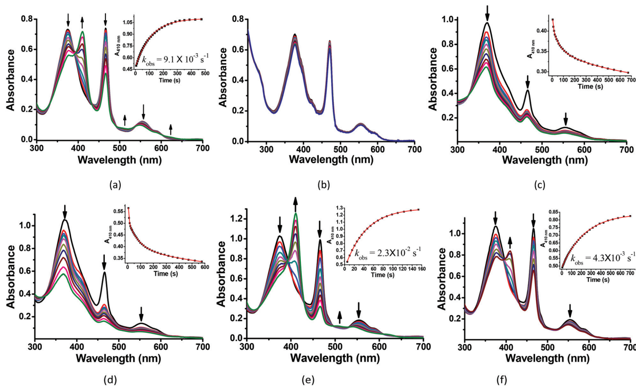
Fig. 2 Kinetic studies of 30 \mu\text{M} (a) His 3 Mn III Mb and (b) wild-type Mn III Mb reacted with 200 equiv. KHSO 5 in PBS buffer (pH = 7.4). And 30 \mu\text{M} His 3 Mn III Mb reacted with 200 equiv. KHSO 5 at (c) pH = 5.1, (d) pH = 6.0, (e) pH = 7.0, and (f) pH = 8.0. Inset: Time course plots of absorbance at ca. 410 nm, attributing to the formation of the Mn=O intermediate.
