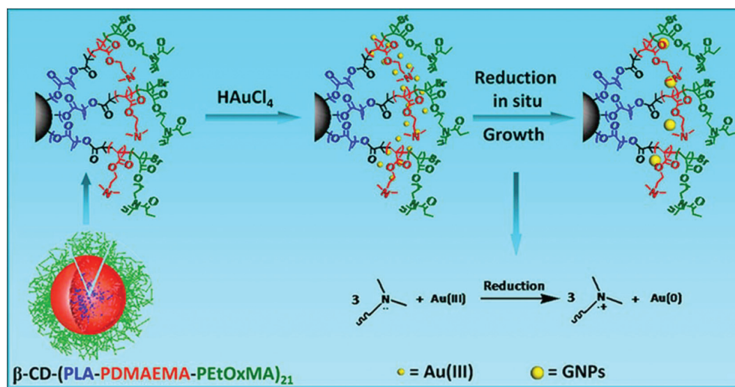
Fig. 19 Schematic representation of using the star-like block copolymer β-CD-(PLA-PDMAEMA-PEToxMA) 21 as a unimolecular micelle template for the synthesis and stabilization of gold nanoparticles. Reproduced with permission from Wiley. 201
