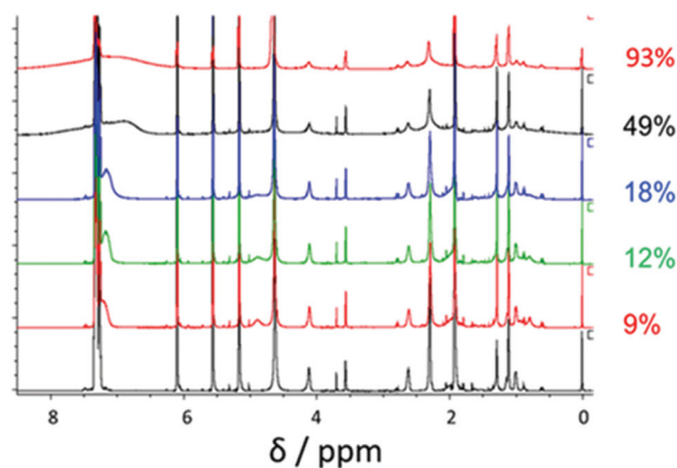
Fig. 2 ^1\text{H} NMR spectra recorded during the RAFT dispersion polymerization of BzMA at 70^\circ\text{C} in \text{d}_6 -ethanol targeting a final diblock composition of PDMA 43 –PBzMA 500 . Monomer conversions were calculated by comparing the integrals of the vinyl monomer to the t = 0 spectrum using TMS as the internal standard.
