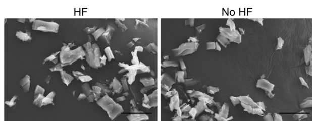
Fig. 1 SEM images of MIL-53(Fe)[H 2 O] synthesized with (left) and without HF (right). The scale bar at the bottom right indicates a length of 20 μm.
