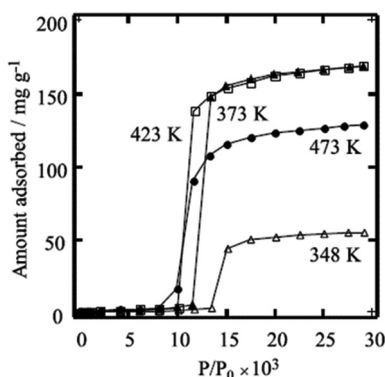
Fig. 16 Gate opening behaviour for \text{CO}_2 adsorption in a Cu(II) MOF. Reproduced with permission from ref. 56, Copyright (2001) Elsevier.
