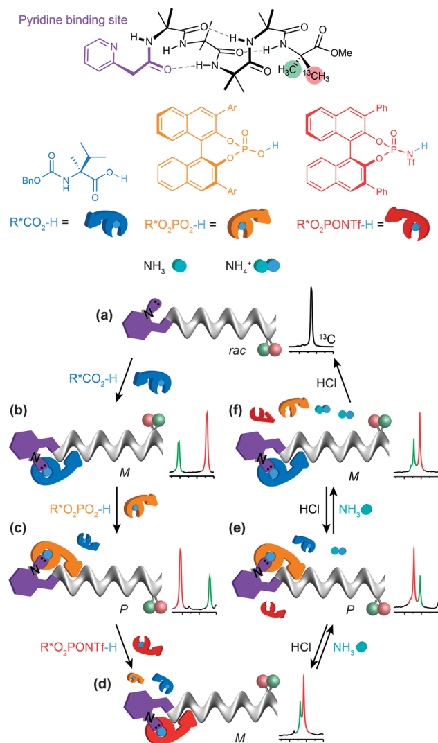
Fig. 12 (a) A dynamic foldamer carrying a ^{13}C NMR reporter of conformational preference and functionalised with a basic pyridine binding site. (b) The dynamic foldamer forms a hydrogen-bonded complex in which a chiral carboxylic acid (blue) induces a conformational preference for left-handed screw sense. (c) A chiral phosphoric acid (orange) induces a right-handed screw sense. (d) A chiral triflamide (red) restores a weak preference for left-handed screw sense. (e) Ammonia disrupts the hydrogen-bonded complex firstly of the most acidic triflamide ligand, then (f) of the phosphoric acid ligand and then finally (g) of the carboxylic acid ligand, returning the receptor to its native form.
