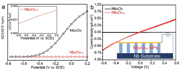
Fig. 3 (a) Mott-Schottky plots of \text{Nb}_2\text{O}_5 and \text{Nb}_2\text{O}_{5-x} NPs films at a frequency of 1 kHz in the dark; (b) comparison of I-V curves of the samples; the inset is the schematic of the measurement.
