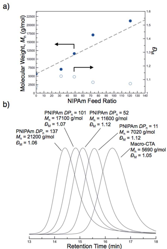
Fig. 2 Molecular weight evolution during the polymerization-induced thermal self-assembly (PITSA) of poly(DMA 3.4 - b -poly(DMA 1.4 - co -AA 6 )- b -polyNIPAm n ) by the chain extension of a macro chain transfer agent containing N,N -dimethylacrylamide (DMA) and acrylic acid (AA), poly(DMA 3.4 - b -poly(DMA 1.4 - co -AA 6 ), with N -isopropylacrylamide (NIPAm). (a) Absolute number-average molecular weight ( M_n ) as a function of NIPAm feed ratio (b) SEC chromatograms as a function of PNIPAm degree of polymerization (PNIPAm DP_n ).
