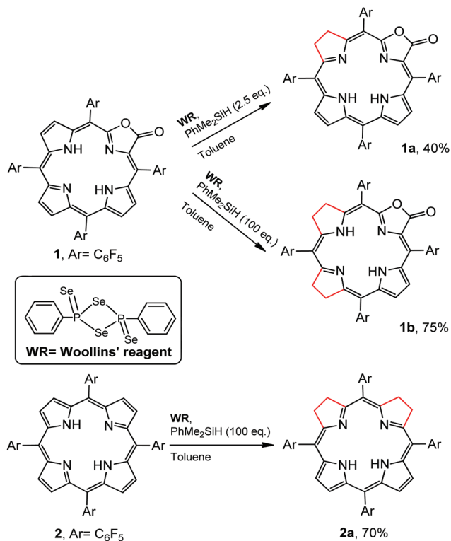
Scheme 2 Synthetic routes for 1a , 1b and 2a .
