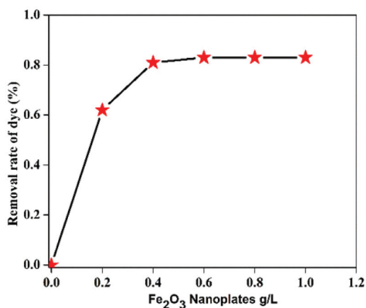
Fig. 7 Effect of concentration of hematite nanoparticles on the photocatalytic degradation of MB.
