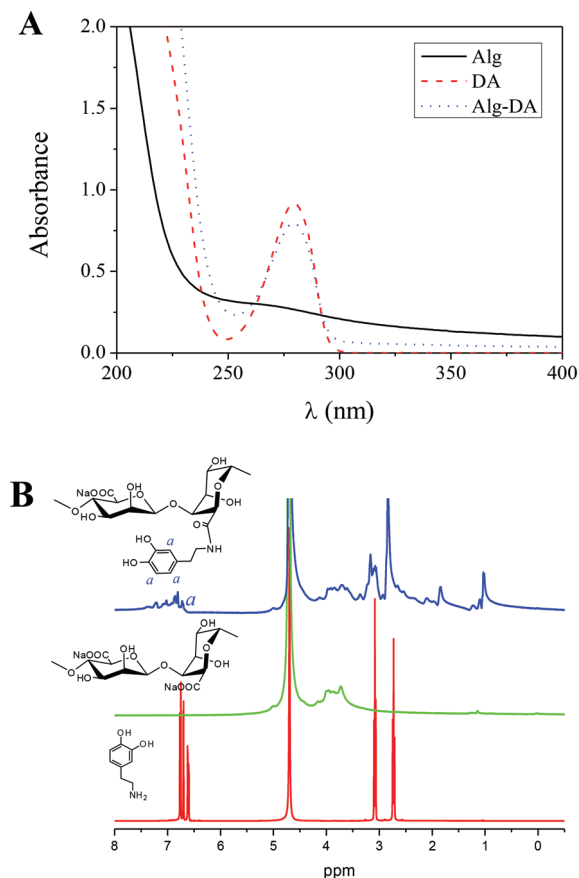
Fig. 1 (A) UV-vis spectra of Alg, DA and Alg-DA conjugate. (B) ^1\text{H} NMR spectra of DA, Alg and Alg-DA conjugate. Solvent: \text{D}_2\text{O} .
