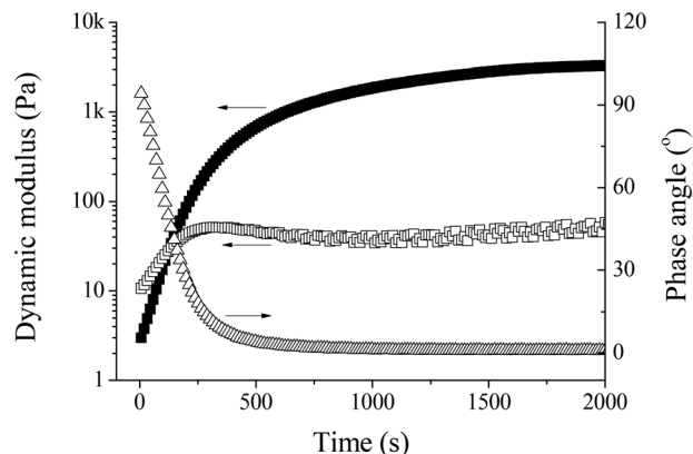
Fig. 3 Evolution of the storage modulus G' (■), loss modulus G'' (□) and phase angle \delta (△) of a 4.0 wt% Alg-DA solution (DS = 21%) with time in the presence of HRP (23.04 U \text{mL}^{-1} ) and \text{H}_2\text{O}_2 (52.0 mM). T = 37^\circ\text{C} .
