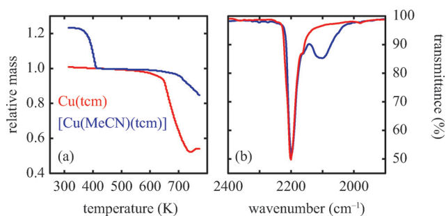
Fig. 5 (a) Thermogravimetric behaviour of Cu(tcm) and [Cu(MeCN)(tcm)]. The mass loss observed near 400 K for the latter corresponds to volatilisation of one molar equivalent of MeCN. Both TGA curves have been normalised to the mass measured at 420 K (b). High-frequency region of the infrared absorption spectra of Cu(tcm) and [Cu(MeCN)(tcm)] showing the emergence of an additional band in the latter, attributed to the nitrile C–N stretch. Colour scheme as in (a).
