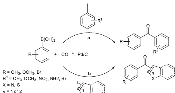
Scheme 45 Reagents and conditions: (a) aryl iodide (1 mmol), arylboronic acid (1.2 mmol), CO (200 psi), 10% Pd/C (2 mol%), K_2CO_3 (3 mmol), anisole (10 mL), 100^\circ C , 8 h; (b) heteroaryl iodide (1 mmol), arylboronic acid (1.2 mmol), CO (200 psi), 10% Pd/C (2.5 mol%), K_2CO_3 (3 mmol), toluene (10 mL), time 10 h, temp. 100^\circ C .
