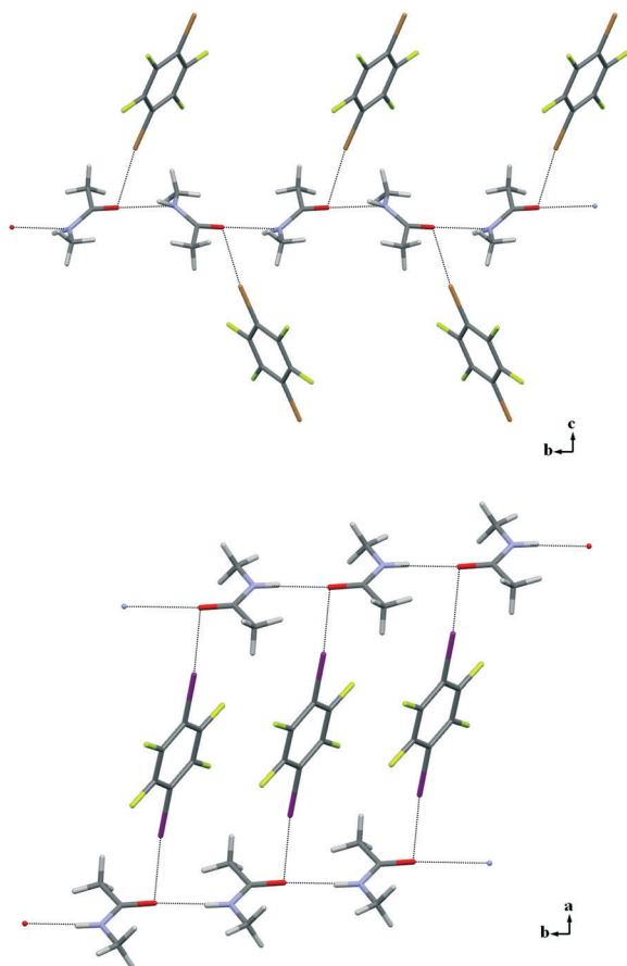
Fig. 2 Partial crystal packing showing how infinite 1D chains (horizontally positioned) formed by NMA via N–H \cdots O HBs further interact with 14DITFB via Br \cdots O XBs in 3c (top) and I \cdots O XBs in 3f (bottom). The disorder on the NMA molecule is omitted for clarity.
