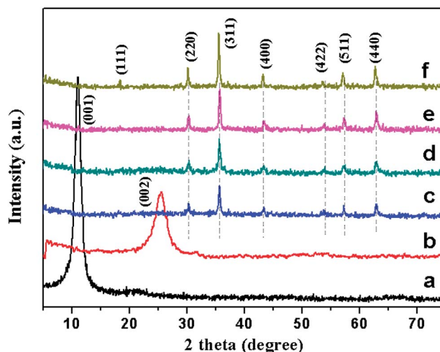
Fig. 2 XRD patterns of GO (a), RGO (b), RGO- \text{Fe}_3\text{O}_4 -1 composite (c), RGO- \text{Fe}_3\text{O}_4 -2 composite (d), RGO- \text{Fe}_3\text{O}_4 -3 composite (e) and \text{Fe}_3\text{O}_4 NPs (f).
