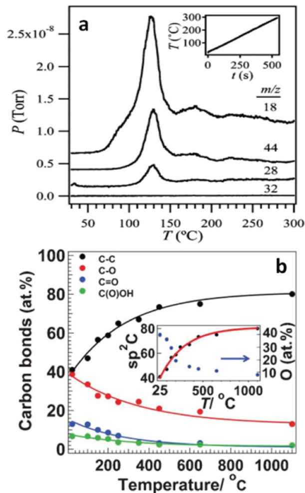
Fig. 14 (a) Temperature programmed desorption spectra of GO film thermally reduced at heating rate of 30 °C min -1 ; m/z = 18, 44, 28, 32 indicate \text{H}_2\text{O} , \text{CO}_2 , \text{CO} , and \text{O}_2 , respectively. The inset is the heating rate curve. Reprinted with permission from ref. 188. Copyright (2009) American Chemical Society. (b) The atomic percentage of different carbon atoms identified by XPS with respect to the annealing temperatures. The inset indicates the oxygen percentage evolution during the reduction process. Reprinted with permission from ref. 106. Copyright (2009) John Wiley and Sons.
