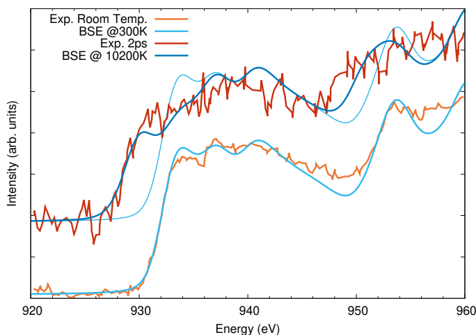
Fig. 5 Cu L_{2,3} edge x-ray absorption calculations compared to measured data taken from Ref. 60. The lower spectra were taken and calculated at room temperature, while the upper spectra, offset vertically for clarity, are at elevated temperature (see text for details). The 300 K calculation is shown a second time with the high-temperature spectra to highlight the shifts in spectral weight with temperature.
