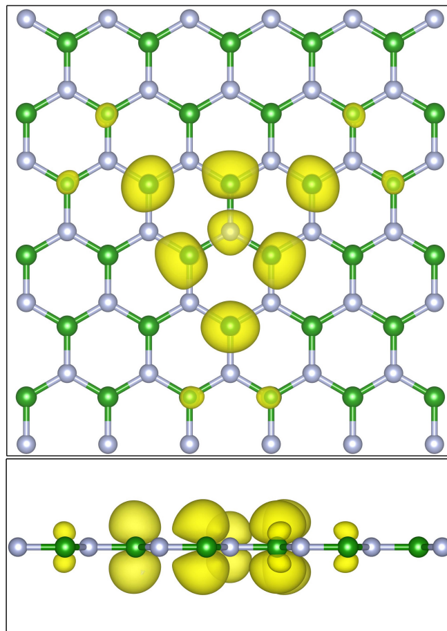
Fig. 4 Top) The excited electron density (yellow) of the lowest energy exciton of a single sheet of hexagonal boron nitride at the nitrogen K edge viewed looking down. Bottom) the same plot but viewed from the side. The absorbing site is the central nitrogen atom (grey). The majority of the electron density is sitting in p_z type states on the first and second nearest neighboring boron atoms (green). Plots generated using VESTA. 56
