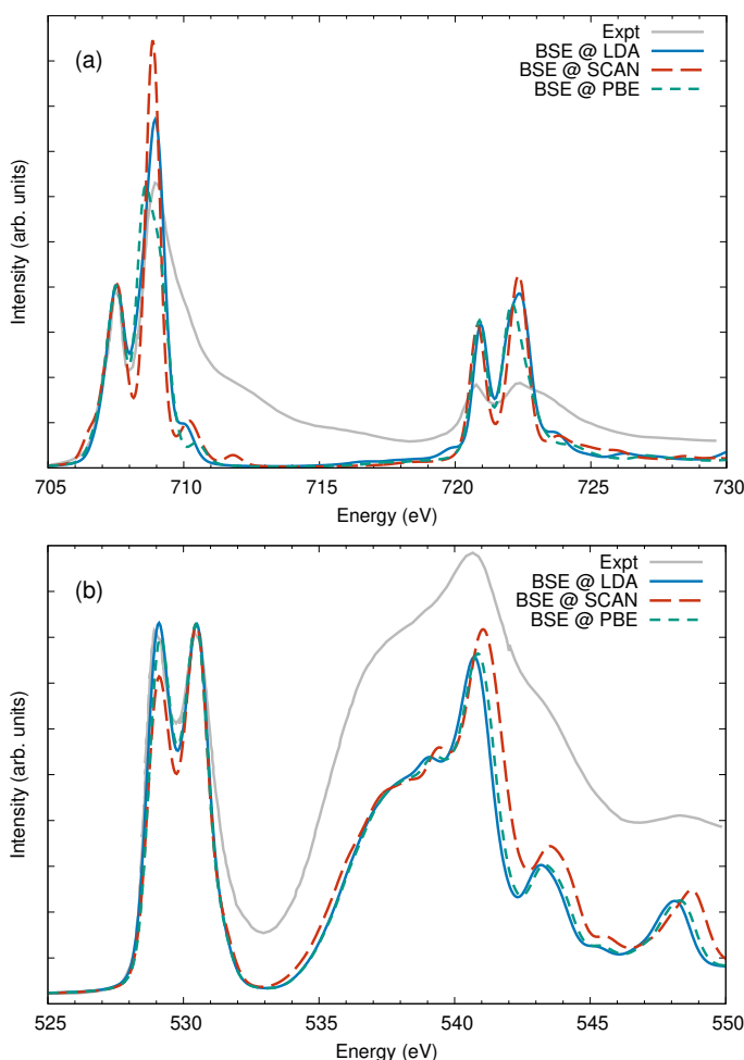
Fig. 7 a) The iron L_{2,3} edge and b) the oxygen K edge of Fe_2O_3 calculated using three different approximations to the DFT exchange correlation potential and compared with experiment from Ref 66. The iron L edges were aligned and scaled to the lowest feature at 707.5 eV and the O K edge to the second feature at 530.5 eV. The differences between the three calculations are minor, however the SCAN potential shows a markedly higher intensity in the e_g orbitals compared to PBE or LDA as can be noted at 530.5 eV or 709 eV.
