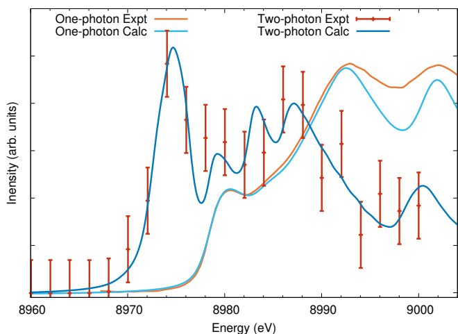
Fig. 6 Cu K edge x-ray absorption calculations compared to measured data taken from Ref. 65 (error bars from the original publication). The two-photon calculated spectra assume a 9 % depopulation of the valence bands, leading to the appearance of a strong pre-edge peak from transitions into the otherwise fully occupied 3d states.
