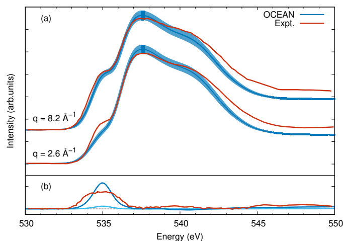
Fig. 10 a) The O K edge of liquid water as seen with NRIXS at momenta of 2.6 \text{ \AA}^{-1} and 8.2 \text{ \AA}^{-1} . Other than the value of the momentum transfer the details of the calculation are the same as for Fig 9, and the experimental data is from Ref 75. b) The difference between the high and low momentum spectra for OCEAN in blue and the measured data in red. For reference, the difference between q = 2.6 \text{ \AA}^{-1} and a dipole XAS calculation is shown in cyan, showing already a slight increase in the pre-edge feature at finite momentum. While the calculated pre-edge appears to be growing faster with increasing momentum in (a) than the measured pre-edge, in (b) it is clear that in the measured data the pre-edge is wider at higher q . The change in the area of the pre-edge is very similar between OCEAN and experiment.
