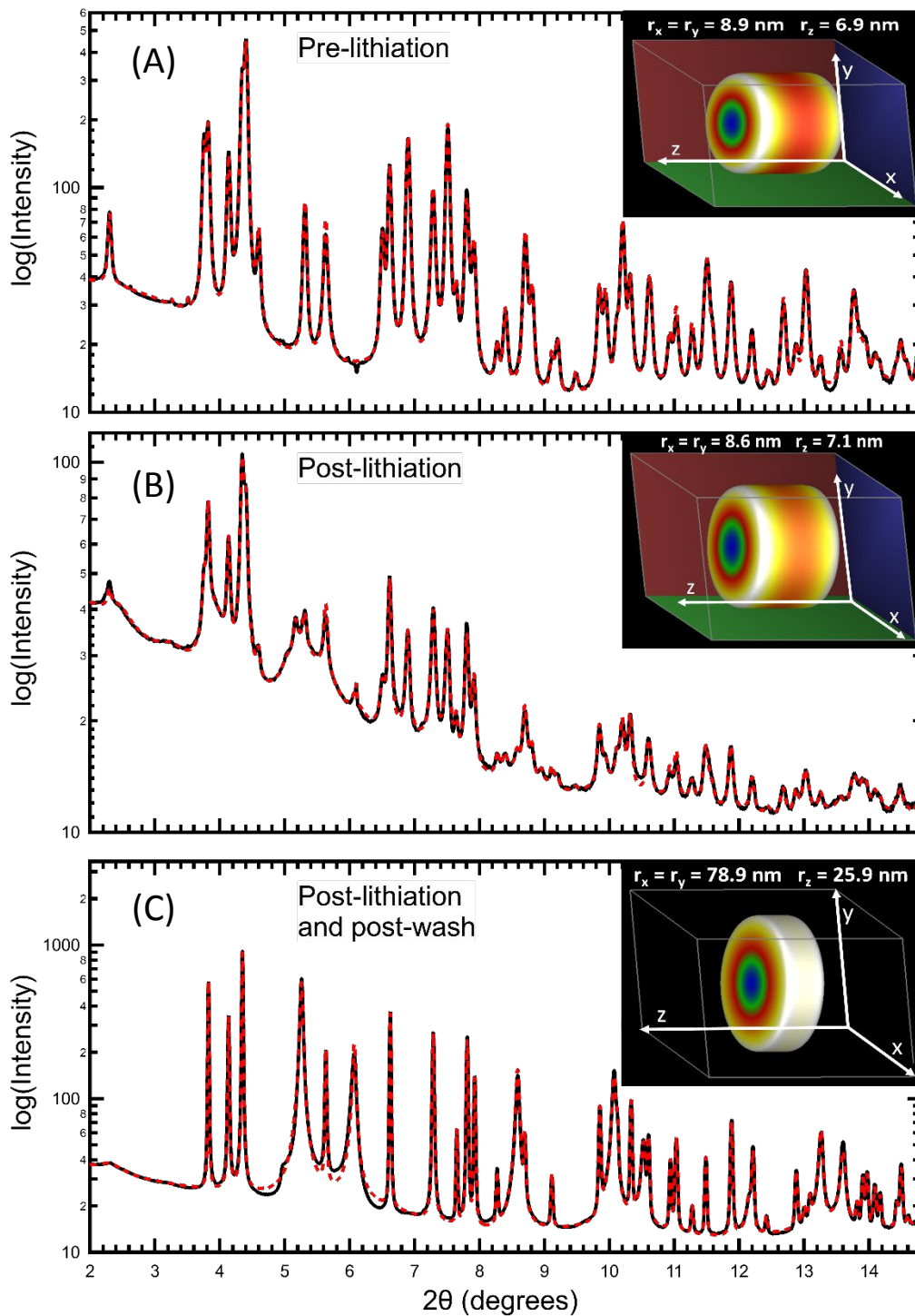
Figure 3. Data fits to synchrotron XRD patterns obtained through Rietveld refinement incorporating anisotropic size broadening of diffraction peaks based on cylindrical particle
