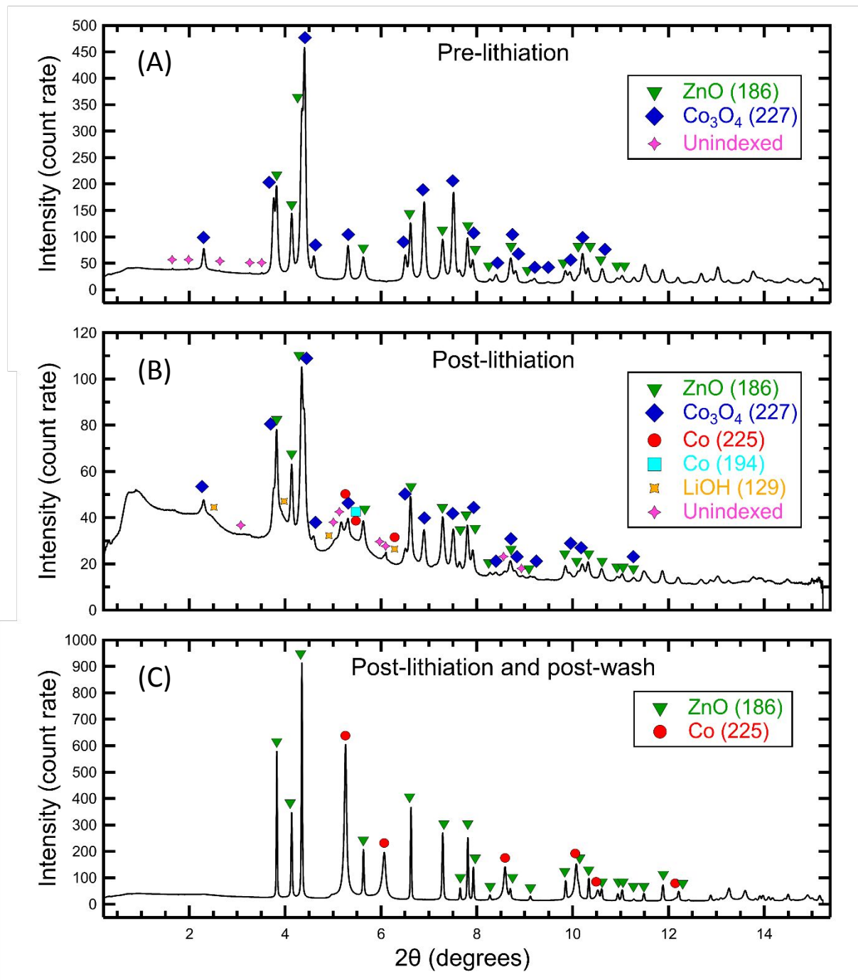
Figure 2. Phase identification results obtained from synchrotron XRD patterns for (a) the pre-lithiation precursor mixture of ZnO and \text{Co}_3\text{O}_4 , (b) the post-lithiation intermediate nanocomposite with a Li-containing phase, and (c) the post-lithiation and post-wash final NPo ZOC product.
