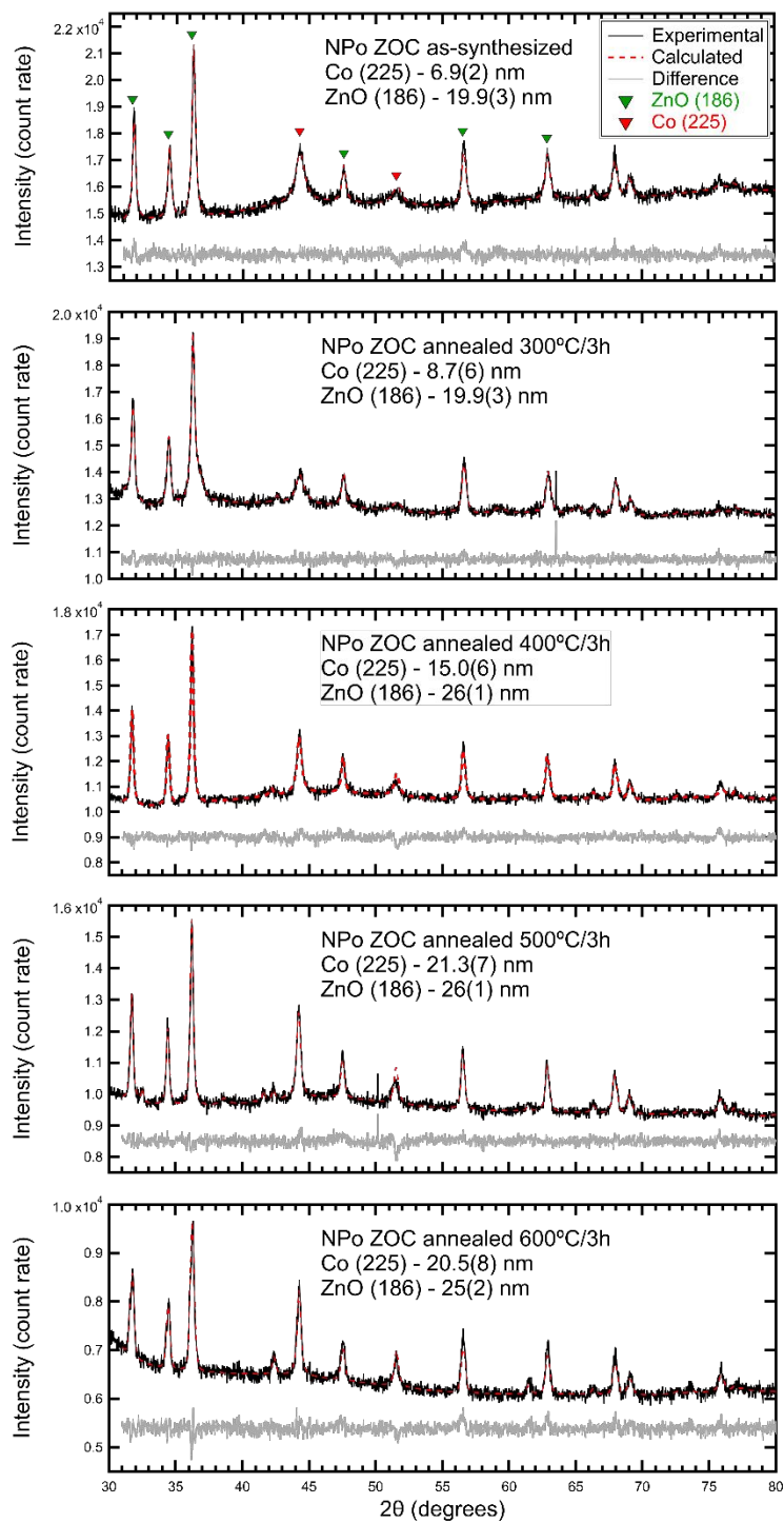
Figure 6. Data fits from Rietveld refinement on XRD patterns of as-synthesized nanoporous ZnO-Co and after annealing for 3 hours at 300 - 600 °C. Further phase information and crystallographic parameters provided in Table S1 .
