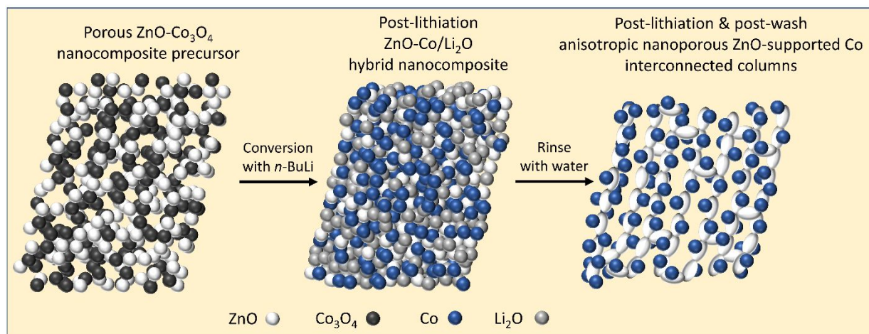
Figure 1. Schematic illustration of Conversion Reaction Synthesis (CRS) of ZOC with an anisotropic particle structure from the co-precipitated ZnO-Co 3 O 4 precursor.
