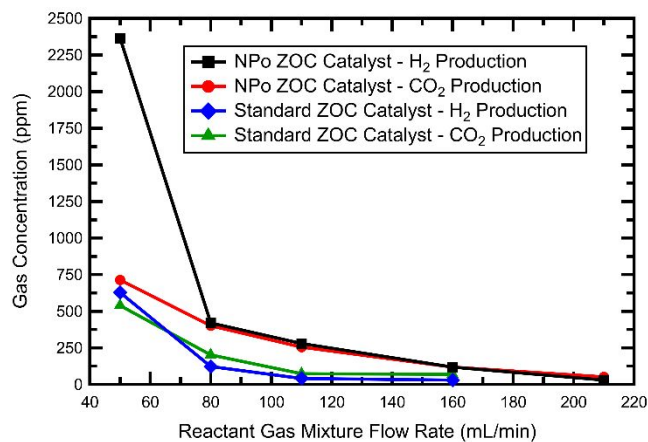
Figure 9. Concentration profiles of H 2 and CO 2 gas produced by steam reformation of ethanol over a ZnO-Co catalyst at various reactant gas mixture flow rates. Tabulated values are summarized in Table S3 .
