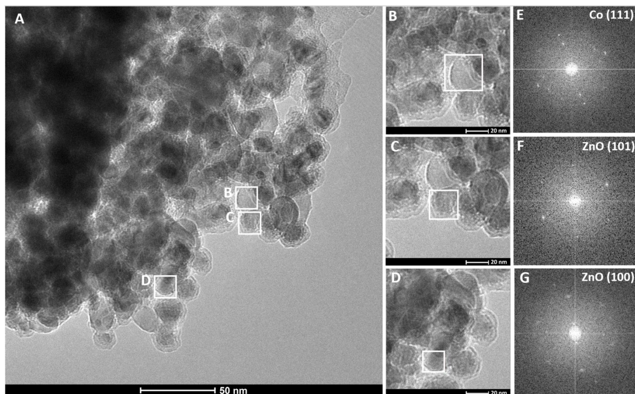
Figure 5. TEM images of post-lithiation and post-wash nanoporous ZnO-supported Co (A). NPo ZOC has primary particles on the order of 20nm, as was suggested by size-strain analysis of XRD data. The zoomed in regions of fcc Co and wurtzite ZnO (B, C, D) show selected area electron diffraction patterns (E, F, G) that confirm the structure of the ZnO and Co phases, as well as their close proximity demonstrating that they are very well intermixed.
