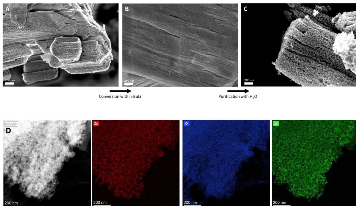
Figure 4. SEM images of (A) pre-lithiation \text{Co}_3\text{O}_4\text{-ZnO} precursor; (B) post-lithiation \text{Co-ZnO-Li}_2\text{O} nanocomposite; (C) post-lithiation and post-wash nanoporous \text{ZnO} -supported \text{Co} . (D) TEM image of post-lithiation and post-wash nanoporous \text{ZnO} -supported \text{Co} as well as the corresponding EDX maps of (from left to right) Zn, O, and Co showing the uniform distribution of the elements within secondary particles. All images have 200 nm scalebars.
