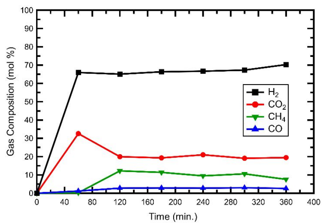
Figure 8. Composition of product gasses when nanoporous ZOC is used as a heterogeneous catalyst for the steam reformation of ethanol over the course of 6 hours. Tabulated values in Table S2 .
