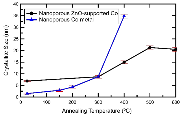
Figure 7. Comparison of temperature dependent coarsening for nanoporous ZnO-supported Co and nanoporous Co metal. Further data on the effect of temperature on surface area can be found in Figure S9.
