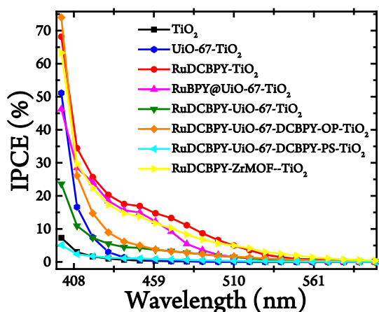
Figure 2. Incident photon to current conversion efficiency (IPCE) spectra of unmodified TiO 2 (black), RuDCBPY on TiO 2 (red), undoped UiO-67-TiO 2 (blue), RuBPY@UiO-67-TiO 2 (pink), RuDCBPY-UiO-67-TiO 2 (green), RuDCBPY-UiO-67-DCBPY-OP-TiO 2 (orange), RuDCBPY-UiO-67-DCBPY-PS-TiO 2 (cyan), and RuDCBPY-ZrMOF-TiO 2 (yellow) collected in a tetrabutylammonium iodide (TBAI) and iodine based electrolyte in CH 3 CN with a platinum counter electrode.
