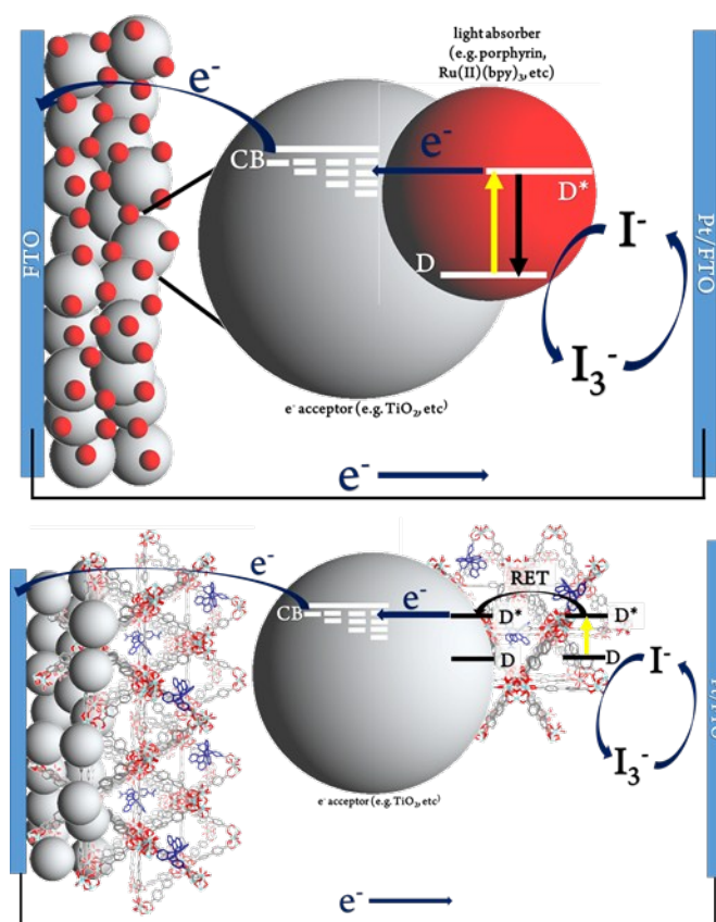
Figure 3. Schematic representation of (top) conventional dye-sensitized solar cell and (bottom) Ru-MOF sensitized solar cells, MOFSCs.
