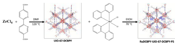
Scheme 2. RuDCBPY-UiO-67-DCBPY-OP.
