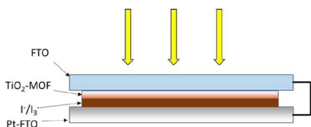
Figure 4. (Left) Front-side solar cell sandwich arrangement used for the photovoltaic cells prepared here. (Right) General scheme depicting the photocurrent generation processes contributing to the observed photocurrent for the RuDCBPY-MOF modified \text{TiO}_2 films. The black arrows indicate charge separation steps whereas the red arrows are indicative of energy transfer/hopping between RuDCBPY centers within the MOF. 1) Charge separation between the BPDC or DCBPY MOF ligands and \text{TiO}_2 . 2) Charge separation between RuDCBPY centers at or within the energy hopping diffusion length from the MOF/ \text{TiO}_2 interface and the \text{TiO}_2 . 3) Non-directional energy transfer/hopping between RuDCBPY centers within the MOF.
