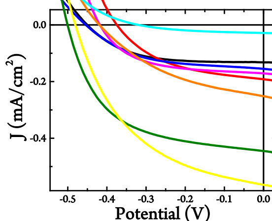
Figure 1. J-V curves of solar cells constructed with bare unmodified \text{TiO}_2 (black), \text{RuDCBPY} on \text{TiO}_2 (red), undoped \text{UiO-67-TiO}_2 (blue), \text{RuBPY@UiO-67-TiO}_2 (pink), \text{RuDCBPY-UiO-67-TiO}_2 (green), \text{RuDCBPY-UiO-67-DCBPY-OP-TiO}_2 (orange), \text{RuDCBPY-UiO-67-DCBPY-PS-TiO}_2 (cyan), and \text{RuDCBPY-ZrMOF-TiO}_2 (yellow) in a tetrabutylammonium iodide (TBAI) and iodine based electrolyte in \text{CH}_3\text{CN} and platinum counter electrode.
