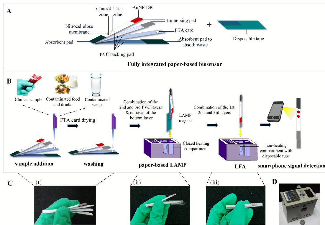
Figure 1. Schematic of an integrated paper-based sample-to-answer biosensor.
