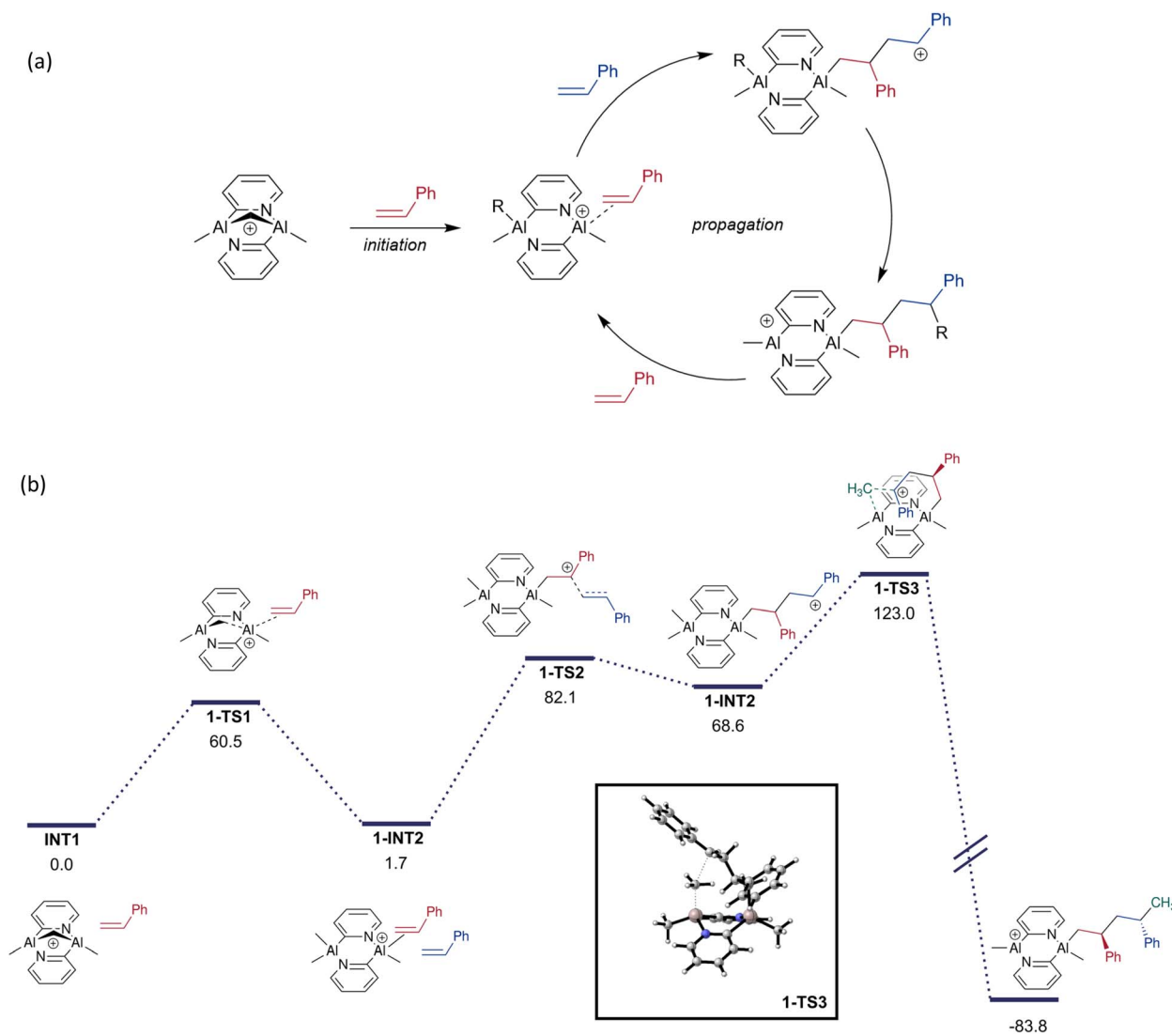
Fig. 9 (a) Viable mechanism involving dimer transfer, and (b) energy profile of the dimer transfer-based polymerisation mechanism (Gibbs free energies in \text{kJ mol}^{-1} ). The TS for the \text{S}_{\text{E}}2 (back) reaction is highlighted in the box.
