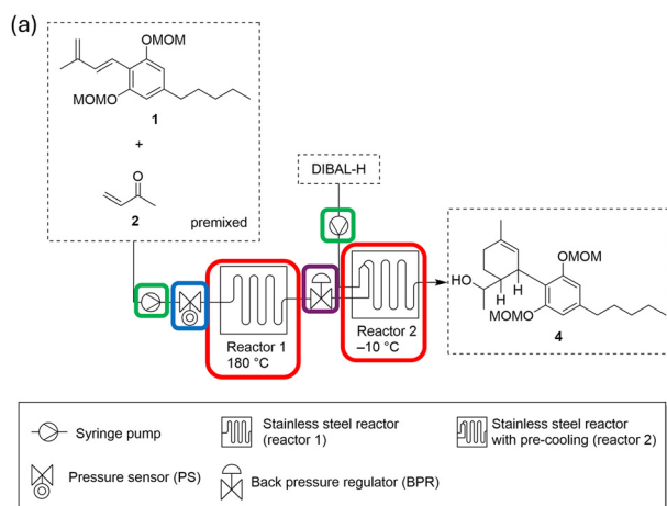
Fig. 8 Scheme (a) and picture (b) of the flow-multistep reaction to 4 .
