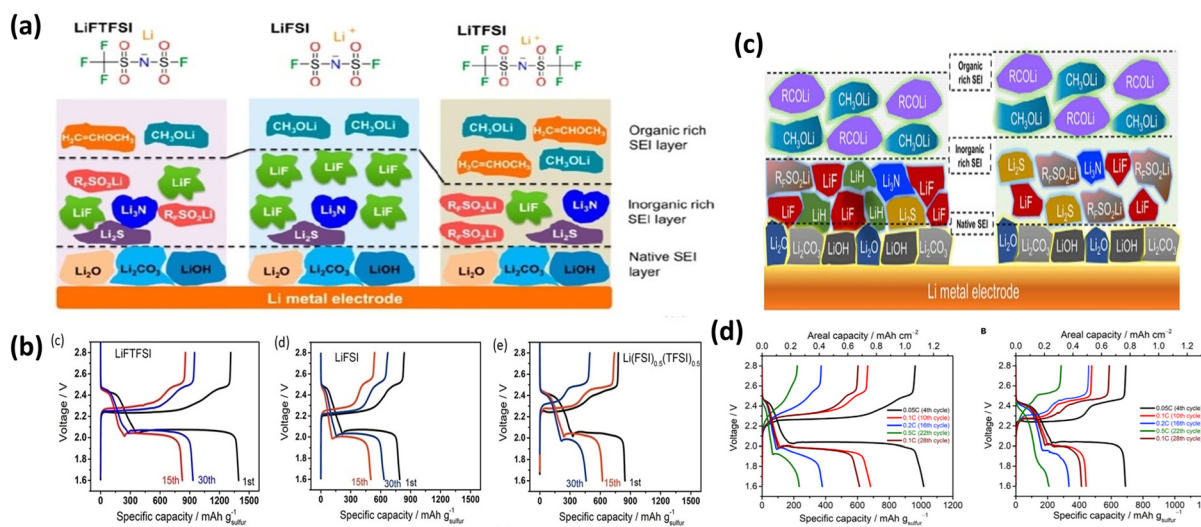
Fig. 10 Interaction of PEO with Li salts with different anions: (a) PEO– \text{LiFTFSI} , PEO– \text{LiFSI} and PEO– \text{LiTFSI} ; (b) charge–discharge plots of salts in (a); (c) SEI layer formed on Li electrode with \text{LiDFTFSI} and \text{LiTFSI} salt; (d) charge–discharge plots of salts in (c). These figures have been reproduced from ref. 52 with permission from American Chemical Society copyright 2018 and from ref. 53 with permission Elsevier copyright 2019.
