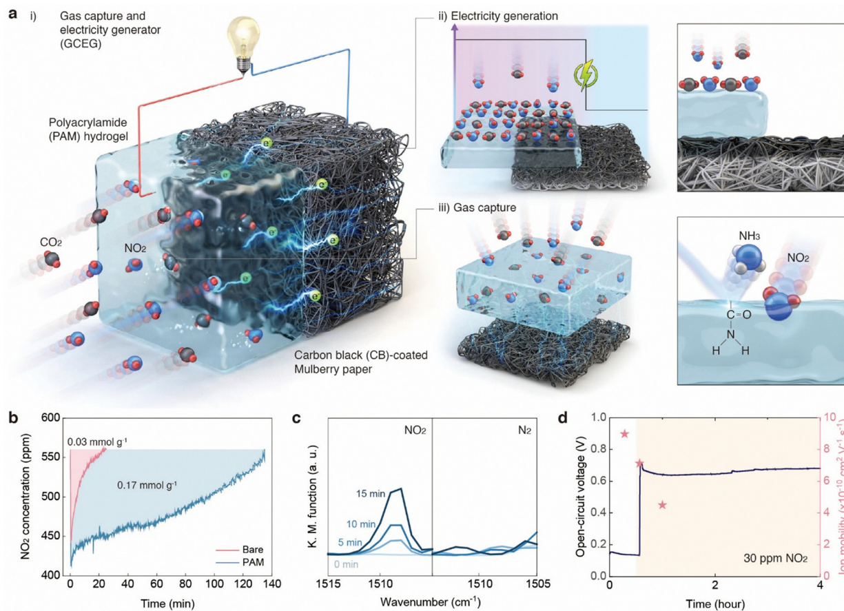
Fig. 1 The gas capture and electricity generator (GCEG) and its main properties. (a) Schematic illustration of the GCEG device, featuring an asymmetric structure with a PAM hydrogel coating on one half of the CB-coated mulberry paper. The device enables electricity generation and gas capture. (b) Adsorption capacity of the PAM hydrogel evaluated under continuous 560 ppm NO 2 exposure. (c) In situ diffuse reflectance infrared Fourier transform spectroscopy (DRIFTS) spectra of the hydrogel after exposure to 1000 ppm NO 2 and N 2 for 15 min at room temperature. (d) Time-dependent V OC of the GCEG under continuous 30 ppm NO 2 exposure at 30% relative humidity (RH), and the corresponding ion mobility changes upon NO 2 exposure as determined by in situ electrochemical impedance spectroscopy (EIS).
