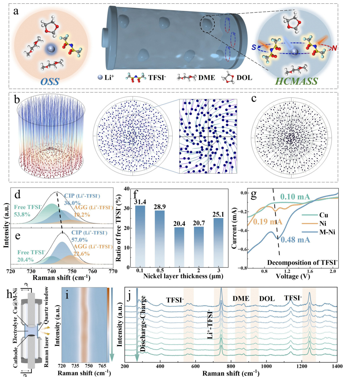
Fig. 2 \text{Li}^+ solvation structure under the action of the M-Ni layer. (a) Schematic diagram of the solvation structures on copper and non-magnetized nickel foil surfaces (yellow), as well as those on magnetized nickel foil surfaces (blue). Simulation results for the different trajectories of \text{Li}^+ during the ion diffusion process (b) with M-Ni and (c) Ni or Cu. Raman spectra of \text{TFSI}^- with (d) Ni and (e) M-Ni. (f) The proportion of free \text{TFSI}^- in the solvated sheath under different magnetized nickel layer thickness conditions. (g) LSV curves of \text{Li}||\text{Cu} cells with various current collectors. (h) Schematic diagram of an in situ Raman test cell. (i) In situ Raman spectra of \text{Li}^+-\text{TFSI}^- during cycles with M-Ni. (j) In situ Raman curves during charging/discharging cycles with M-Ni.
