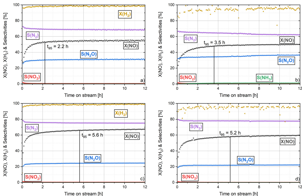
Fig. 6 Long-term trends of NO, \text{H}_2 conversion, and product selectivities of 1%Pd/TiO 2 /HY (a and b) and 1%Pd/TiO 2 /HY + Fe-BEA (2:1, m:m) (c and d) in the dry gas mixture (a and c: 1000 ppm NO, 5000 ppm \text{H}_2 , 10 vol% \text{O}_2 in \text{N}_2 ) and humid gas mixture (b and d: +5 vol% \text{H}_2\text{O} ) at a GHSV = 75 000 \text{h}^{-1} and T = 200 °C.
