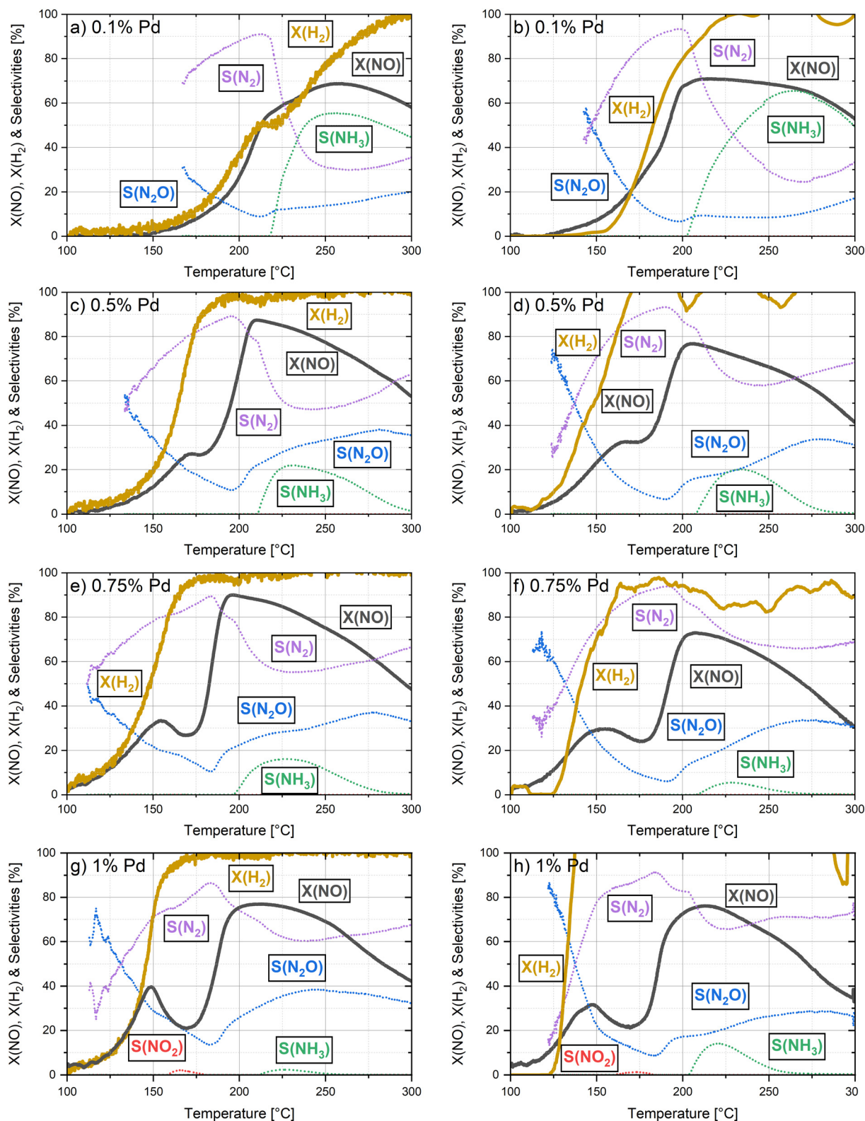
Fig. 1 NO and H 2 conversion (solid lines) and product selectivities (dotted lines) during the light-off measurements of the x\% Pd/TiO 2 /HY catalysts with x = 0.1 (a and b), 0.5 (c and d), 0.75 (e and f), and 1 (g and h) in the dry gas mixture (a, c, e and g; 1000 ppm NO, 5000 ppm H 2 , 10 vol% O 2 in N 2 ) and humid gas mixture (b, d, f and h; +10 vol% H 2 O); GHSV = 60 000 h -1 .
