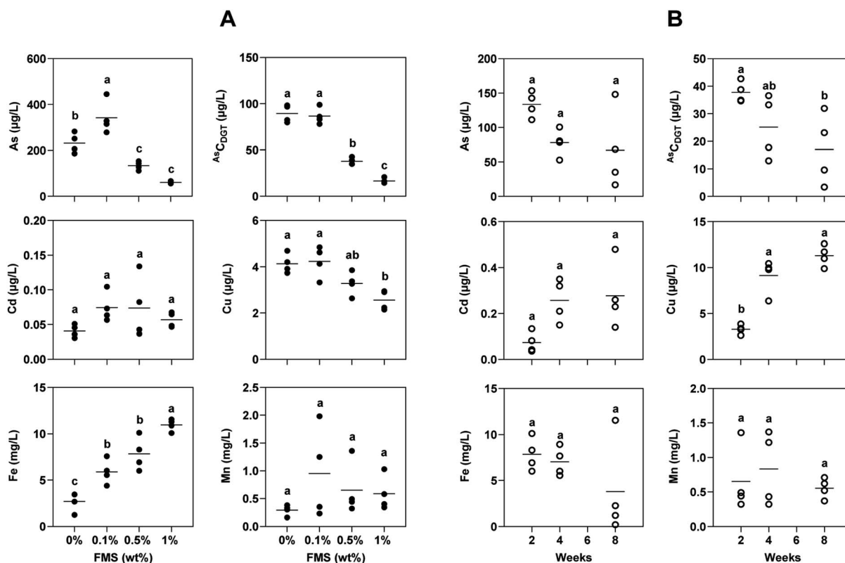
Fig. 4 Effect of FMS on element concentration in soil pore-water ( C_{sol} ) and DGT measured As ( As_{DGT} ) (Mean, n = 4 ). (GLM, post hoc analysis was carried out using Tukey Pairwise Comparisons). Different letters above each bar represent significant differences between treatments ( P < 0.05 ). (A): Dose. (B): Time.
