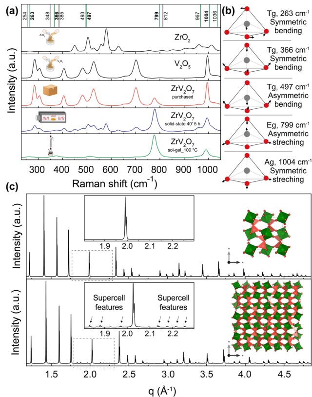
Fig. 7 (a) Raman spectra of \text{ZrV}_2\text{O}_7 synthesised via sol-gel (sol-gel _{100^\circ\text{C}} route (green), 40' 5 h solid-state reaction (blue) and purchased material (red). These spectra are compared with \text{V}_2\text{O}_5 and \text{ZrO}_2 reagents. The purchased material mostly matches \text{V}_2\text{O}_5 spectra, while the solid-state reaction product shows a combination of peaks representing both oxides and \text{ZrV}_2\text{O}_7 . Vertical lines represent simulated Raman positions. Vibrations marked in green contribute to the Raman spectra and match the sol-gel reaction product within the margin of error. (b) Vibrations that correspond to 263, 366, 497, 799, and 1004 \text{cm}^{-1} frequencies are visualised above in a schematic way. Animations showing these vibrations are provided in the ESI.† (c) The XRD pattern of the \text{ZrV}_2\text{O}_7 structure used for computational simulations (c top) compared with the room temperature superstructure used in structure refinements (c bottom).
