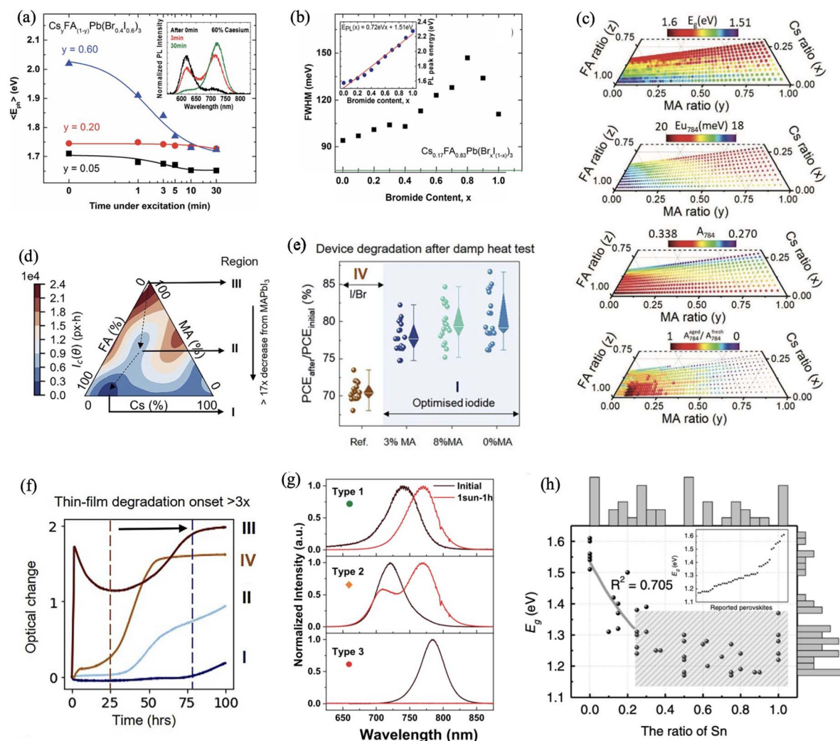
Fig. 1 (a) Changes in average PL emission photon energy ( E_{ph} ) of \text{Cs}_y\text{FA}_{1-y}\text{Pb}(\text{Br}_{0.4}\text{I}_{0.6})_3 films at y = 0.05 , y = 0.20 and y = 0.60 . (b) FWHM of the PL emission spectra of \text{Cs}_{0.17}\text{FA}_{0.83}\text{Pb}(\text{Br}_{x(1-x)})_3 films as a function of \text{Br}^- content x . Inset shows the correlation between PL peak energy and \text{Br}^- content with fitting function. Reproduced from ref. 62 with permission from The Royal Society of Chemistry, copyright 2017. (c) Ranges of bandgap ( E_g ), Urbach energy ( E_{u784} ), absorbance ( A ) and aged to fresh absorbance ratio ( A_{\text{aged}784}/A_{\text{fresh}784} ) of \text{Cs}_x\text{MA}_y\text{FA}_z\text{PbI}_3 alloys at 520 nm locations. Reproduced from ref. 63 with permission from Wiley-VCH GmbH, copyright 2023. (d) Non-linear instability landscape ( I_c(\theta) ) within the \text{Cs}_x\text{MA}_y\text{FA}_{1-x-y}\text{PbI}_3 compositional space with stability in the order of Region I > Region II > Region III. (e) Comparison of percentage ratios of PCEs after damp heat degradation tests between Region IV I/Br-based PSCs and Region I I-based PSCs. (f) Optical changes as a function of degradation time showing Region I as the most stable region. Reproduced from ref. 34 with permission from Elsevier Inc., copyright 2021. (g) Normalized PL peaks of the photodegradation of materials showing three different degradation pathways denoted as Type 1, Type 2 and Type 3. Reproduced from ref. 21 with permission from Elsevier Inc., copyright 2023. (h) Fitted plot of bandgap ( E_g ) as a function of Sn : Pb ratio for 43 reported perovskites and histograms indicating corresponding distributions with respect to Sn : Pb ratio and bandgap. Inset is the bandgap values of the perovskites in ascending order. Reproduced from ref. 77 with permission from Springer Nature Ltd, copyright 2022.
