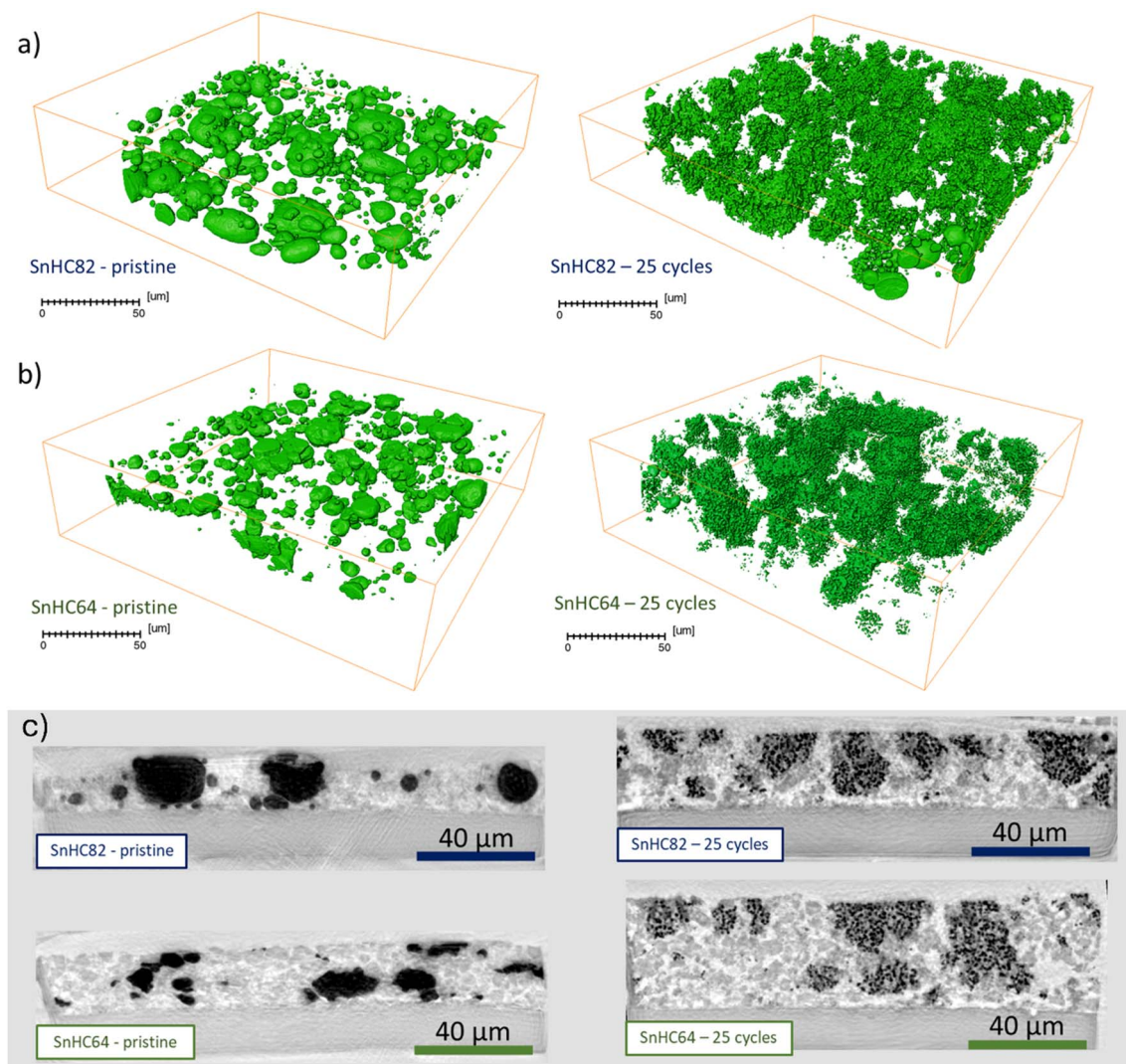
Fig. 5 Observation of the spatial distribution of Sn particles from phase contrast XCT of a 150 \mu\text{m} wide, 150 \mu\text{m} deep area of the pristine and cycled (a) SnHC82 and (b) SnHC64 electrodes (100 nm resolution images). (c) Orthogonal slice views of the SnHC82 and SnHC64 pristine and cycled electrodes.
