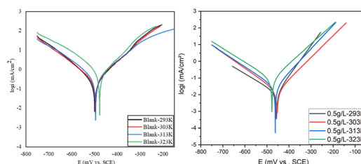
Fig. 9 The PDP plots of MS in 1 M HCl + 0.5 \text{ g L}^{-1} of the mixture at different temperatures.
