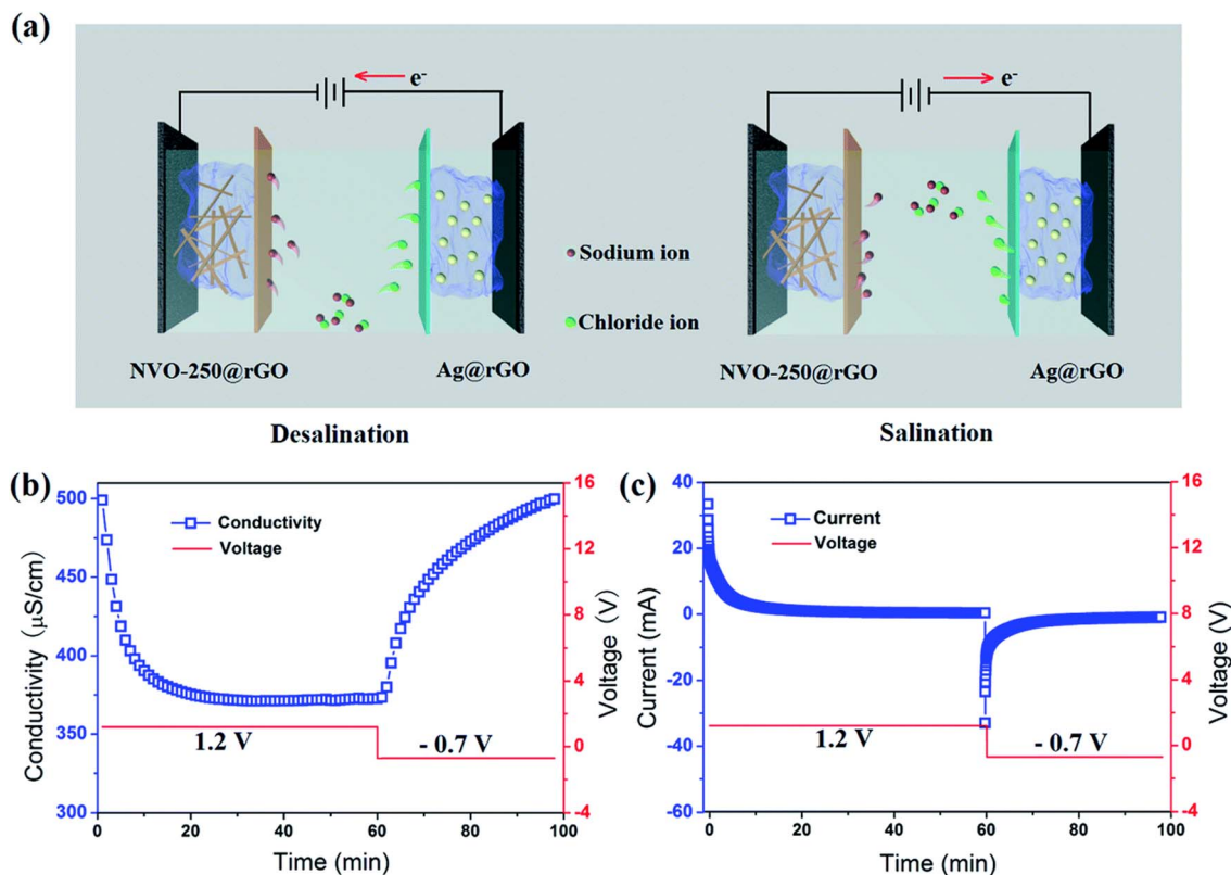
Fig. 10 Working mechanism, conductivity characterization, and current transient response of the binary high-capacity electrochemical system Ag@rGO||NVO-250@rGO in the 1.2 V/500 μS cm -1 NaCl system. 90 (a) Working mechanism of Ag@rGO||NVO-250@rGO Di-HCDI system, (b) conductivity and (c) current transient of the Ag@rGO||NVO-250@rGO Di-HCDI system in 500 μS cm -1 NaCl solution at 1.2 V.
