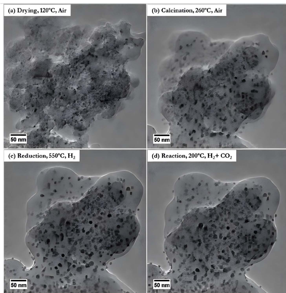
Fig. 13 IL-TEM images of the \text{GaPd}_2/\text{SiO}_2 catalyst acquired after drying (a), calcination (b), reduction (c), and methanol synthesis (d). 333 Copyright 2015 American Chemical Society.
