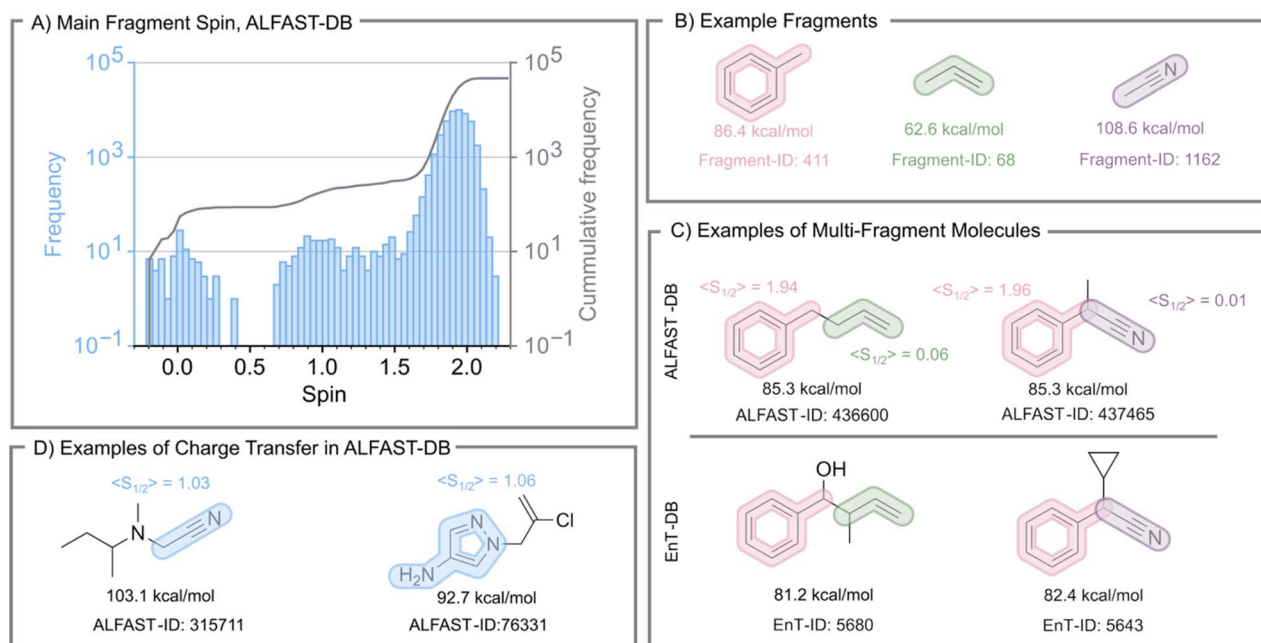
Fig. 4 (A) Absolute (blue histogram) and cumulative frequency (grey line) of the distribution of the main fragment's spin within the ALFAST-DB. (B–D) Example DFT-computed S_0 – T_1 adiabatic gaps for fragments and for multi-fragment molecules within the ALFAST-DB and the EnT-DB. The spin of each fragment was computed from the atomic Mulliken Spin Densities. The example fragments (B) were computed at the same theory level as ALFAST-DB. We note that the EnT-Database does not explicitly include an ID number for each molecule; ID numbers were assigned in this work for organization.
