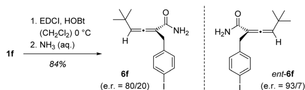
Scheme 5 Proof of absolute configuration: Enantioenriched carboxylic acid was converted into amide 6f (EDCI = 1-ethyl-3-(3-dimethylaminopropyl)carbodiimide, HOBT = 1-hydroxybenzotriazole) which was compared on chiral HPLC with a sample of amide ent - 6f , 12c the absolute configuration of which was known.
