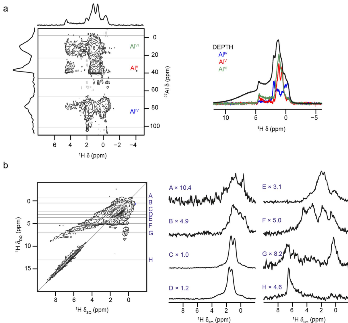
Fig. 11 (a) ^1\text{H} - ^{27}\text{Al} (14.1 T, 40 kHz) D-HMQC spectrum (with TRAPDOR recoupling) of \gamma - \text{Al}_2\text{O}_3 dehydrated at 550 ^\circ\text{C} , with sum projections (extracted parallel to \delta_2 ) over the regions corresponding to Al IV , Al V and Al VI (as shown), overlaid with the ^1\text{H} DEPTH (14.1 T, 40 kHz) DEPTH MAS NMR spectrum of \gamma - \text{Al}_2\text{O}_3 dehydrated at 550 ^\circ\text{C} . (b) ^1\text{H} (14.1 T, 40 kHz) DQ MAS spectrum (acquired using BABA recoupling) of \gamma - \text{Al}_2\text{O}_3 dehydrated at 550 ^\circ\text{C} , with cross sections (extracted parallel to \delta_2 and vertically expanded as shown) extracted at the \delta_1 positions indicated. For detailed experimental parameters see Section S1 of the ESI.†
