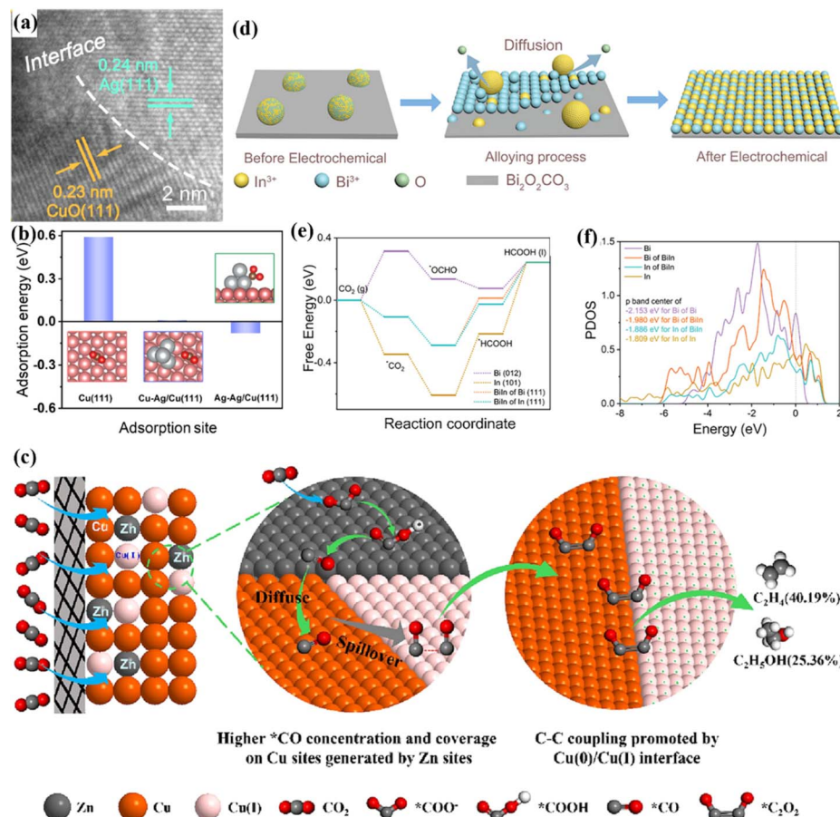
Fig. 19 (a) HRTEM image. (b) The adsorption energy of \text{CO}_2 on the surface of different catalysts. Reproduced with permission. 113 Copyright 2024, Elsevier Ltd. (c) The reaction mechanism diagram on CuZn/GDE. Reproduced with permission. 114 Copyright 2024, Elsevier Ltd. (d) A schematic diagram of atomic movement under electrolysis conditions. (e) The free energy diagrams of HCOOH on different interfaces. (f) PDOS image. Reproduced with permission. 115 Copyright 2023, Wiley-VCH.
